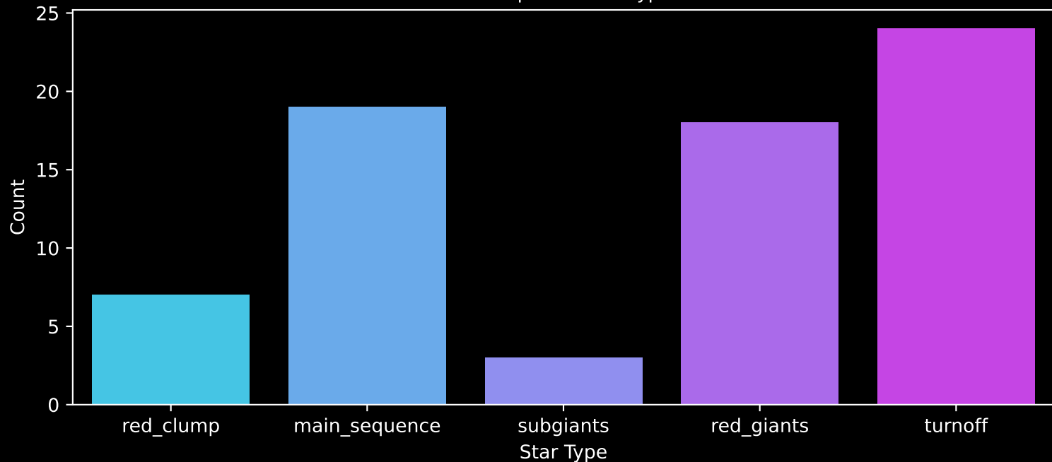
GALAH DR4 Field: [7358] Count plot of Star Type
