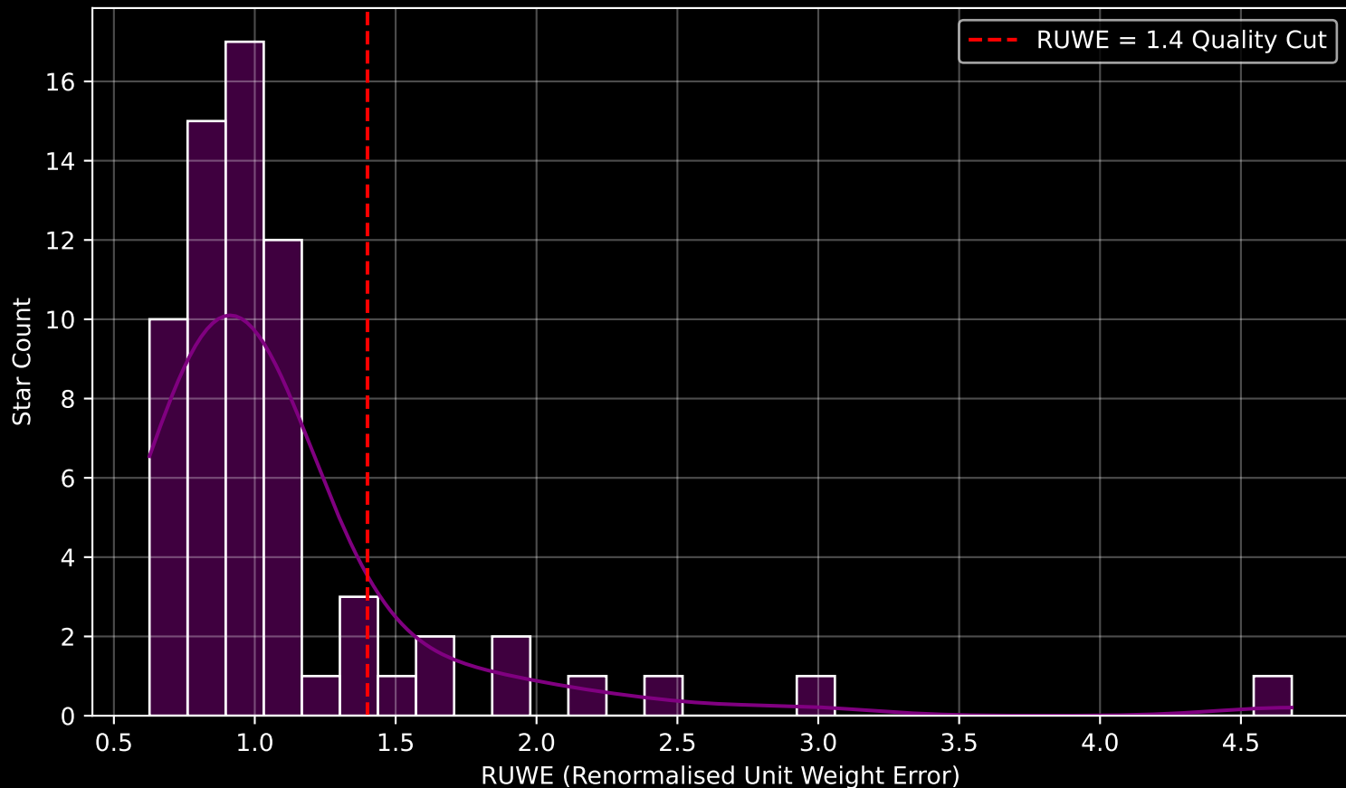
GALAH DR4 Field [7358] RUWE Distribution (n= 67)
