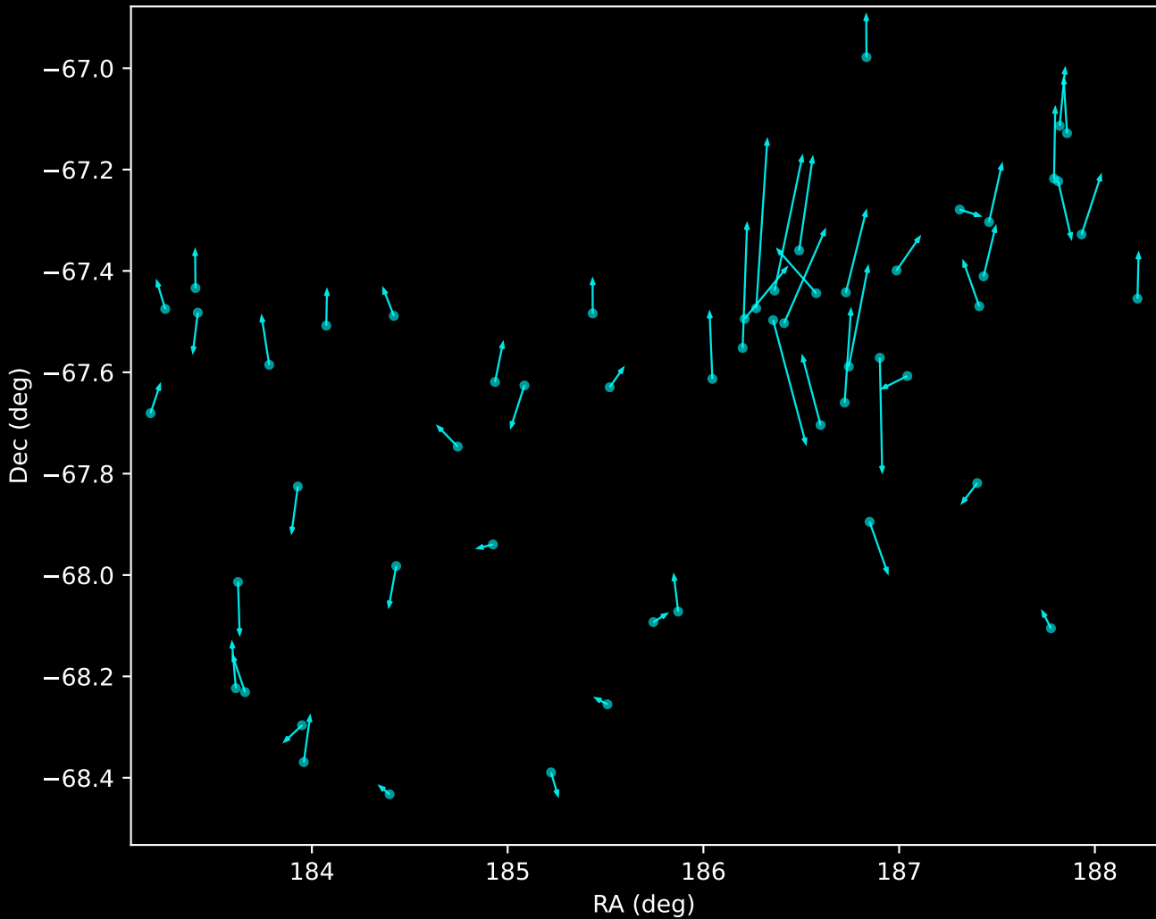
GALAH DR4 Noise Stream Proper Motion Vectors (n=55)
